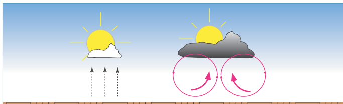
Convection
